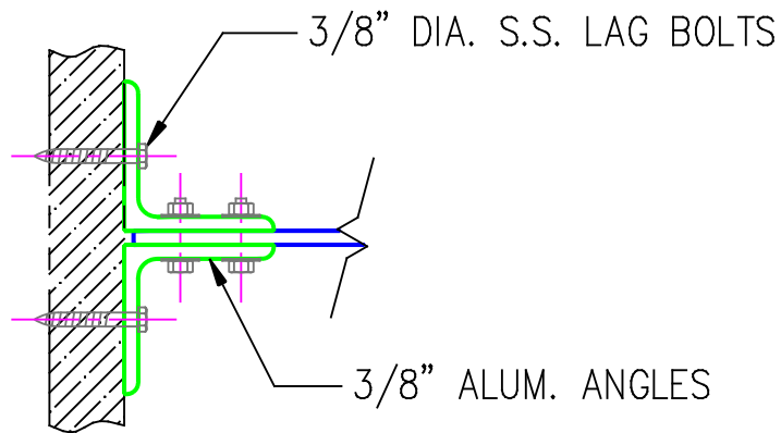
STANDARD MOUNTING ~ TOP VIEW (ALTERNATE MOUNTING STYLES AVAILABLE)
